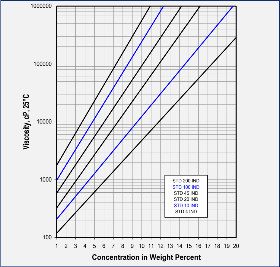
Viscosity in Terpeneol
